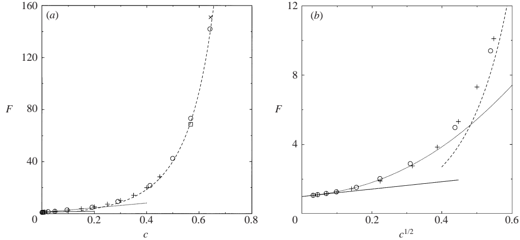
FIGURE 3. (a) The non-dimensional Stokes-flow drag force on the spheres in random arrays as a function of the solid volume fraction: O, lattice-Boltzmann simulations whose parameters and statistical errors are listed in table 1; +, the multipole simulations of Ladd (1990); \square , a lattice-Boltzmann simulation of Stokes flow in a cylindrical packed bed of spheres by Maier et al. (1998); \times , the experiments of Fand et al. (1987). The solid line is the O(c^{1/2}) theory of Brinkman 1947, the dotted line is Brinkman's theory with corrections up to O(c) (10) (Kim & Russel 1985), and the dashed line is the Carman correlation (11) (Carman 1937). (b) As (a) but with the axes scaled to detail the limit of vanishing solid volume fraction.
